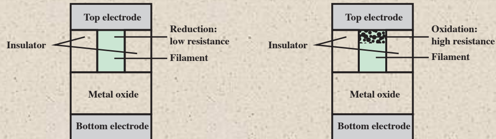
(c) ReRAM
